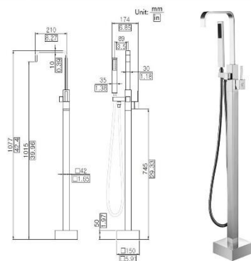
KF-2007 FREESTANDING FAUCET IN CHROME
